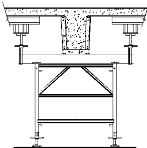
GARAGE BEAM
