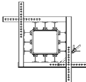
HD COLUMN SYSTEMS
