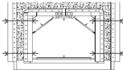
BOX CULVERT SYSTEMS
