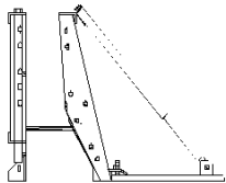
BARRIER RAILS
