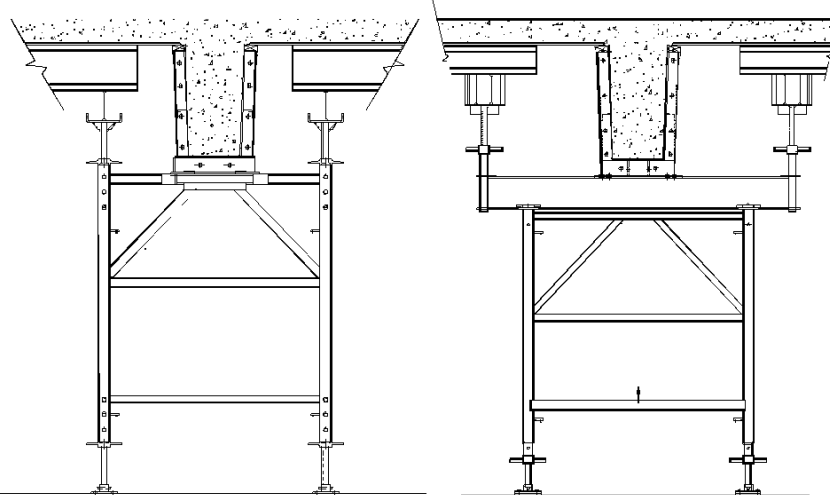
CONVENTIONAL LAYOUT
